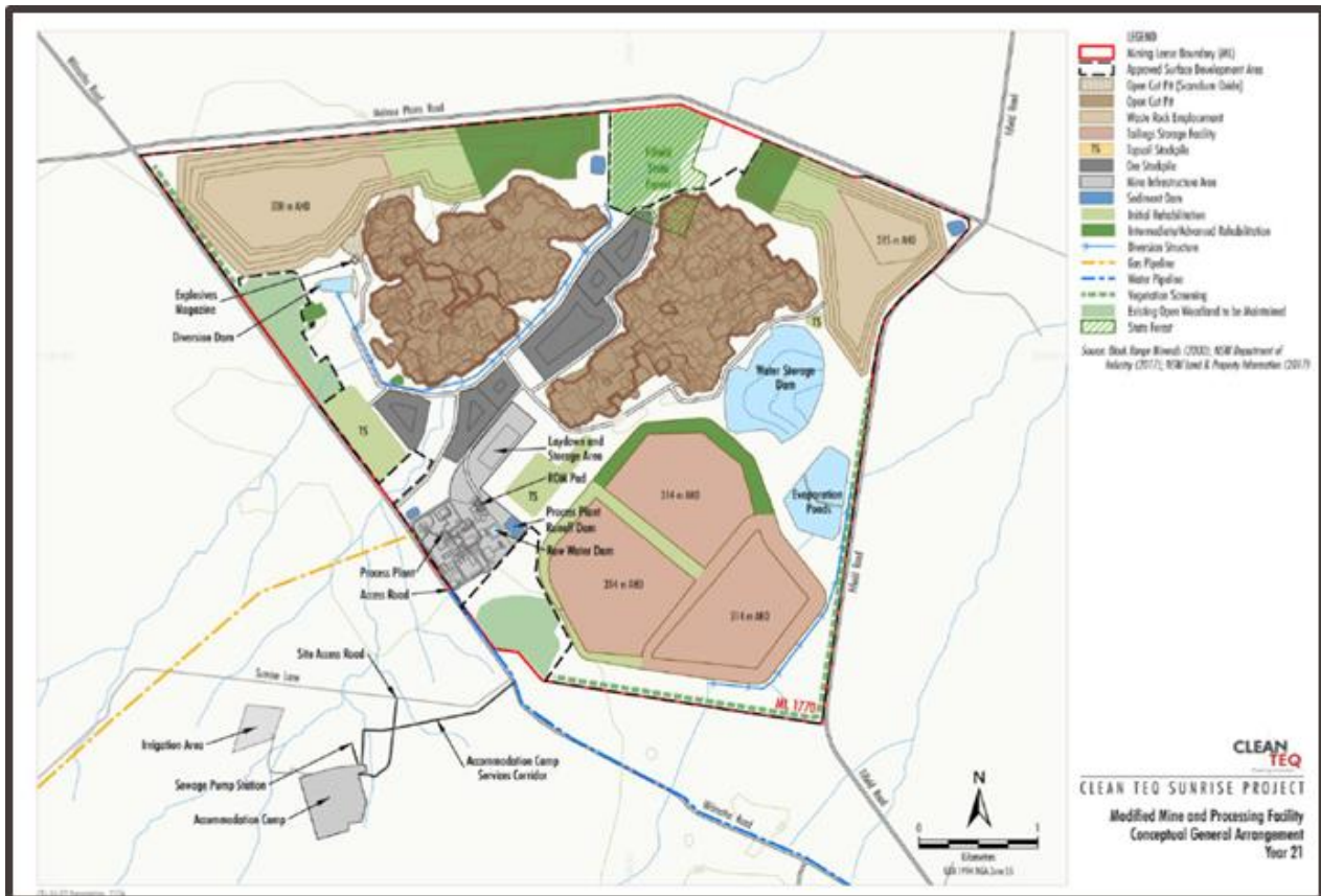
The approved Clean TeQ Sunrise mine and processing facility
