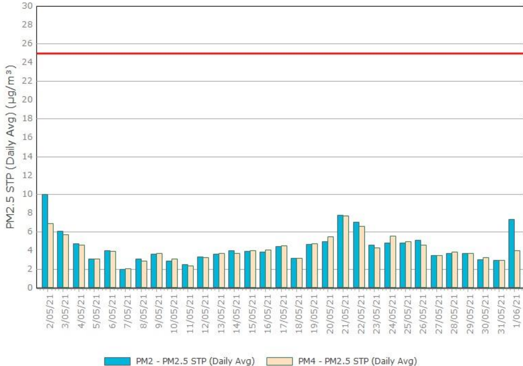
Figure 3. PM2.5 (24 hr Average) with Compliance Criteria – May 2021
