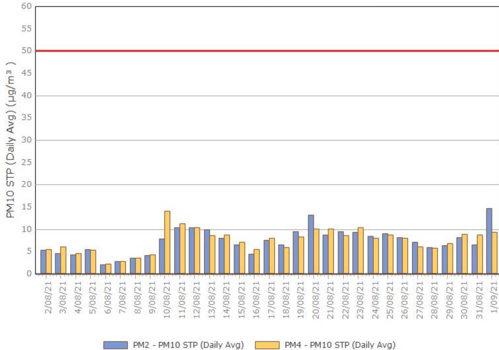
Figure 2. PM10 (24 hr Average) with Compliance Criteria – August 2021
