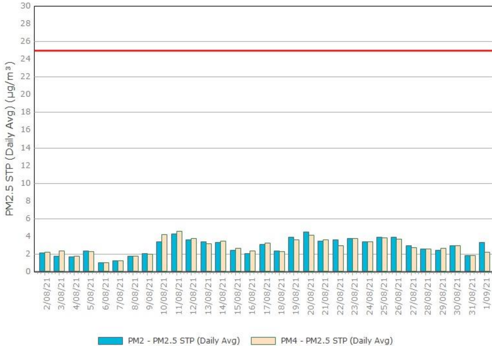
Figure 3. PM2.5 (24 hr Average) with Compliance Criteria – August 2021
