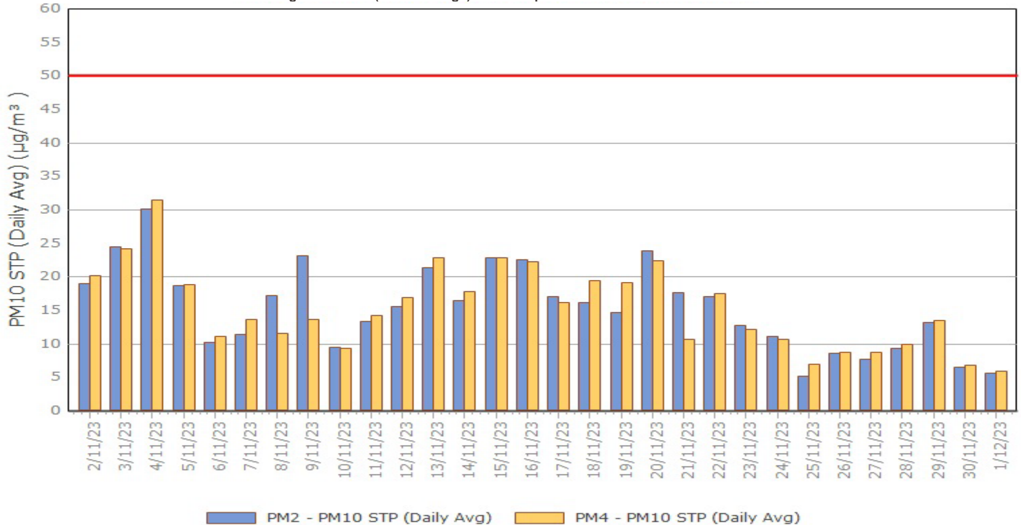
Figure 2. PM10 (24 hr Average) with Compliance Criteria – November 2023
