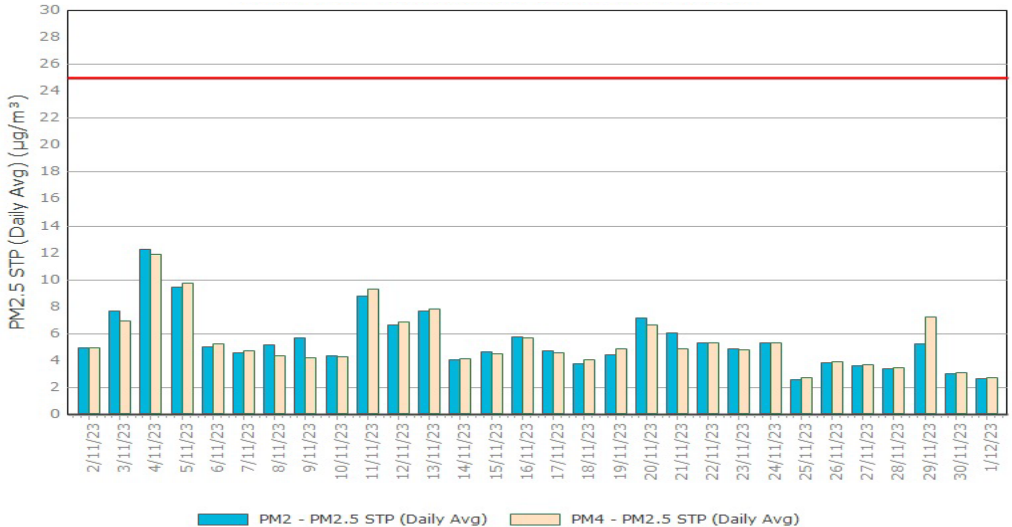
Figure 3. PM2.5 (24 hr Average) with Compliance Criteria – November 2023
